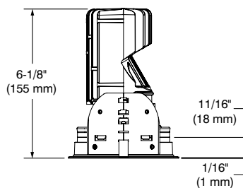
WITH FLANGE
